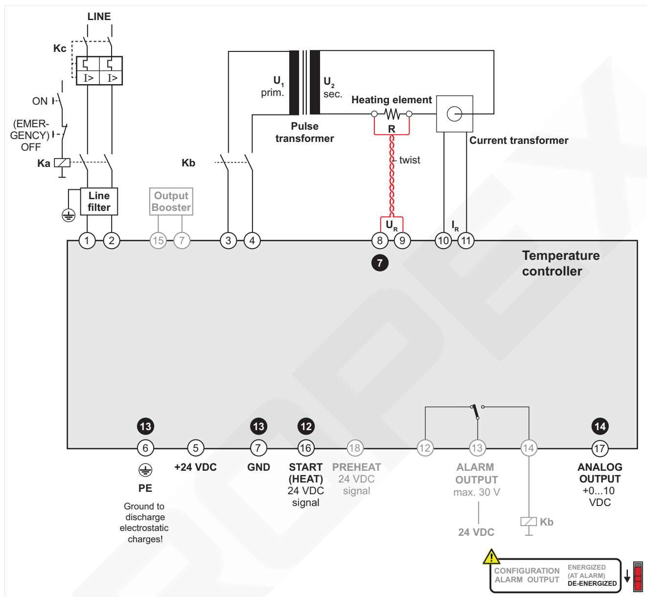
Illustration 1: Comparison of RES-401 and RES-5008 terminal assignment
